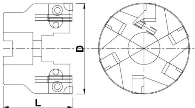
PCD Brazed Face Milling Cutter (mm)
