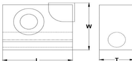
PCD Brazed Face Milling Cutter Cartridge (mm)
